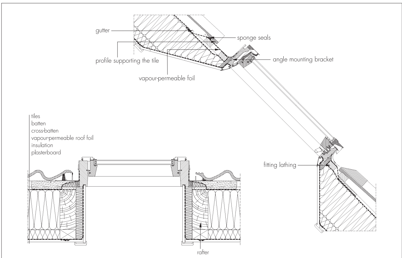
Figure 3 Typical window placements
