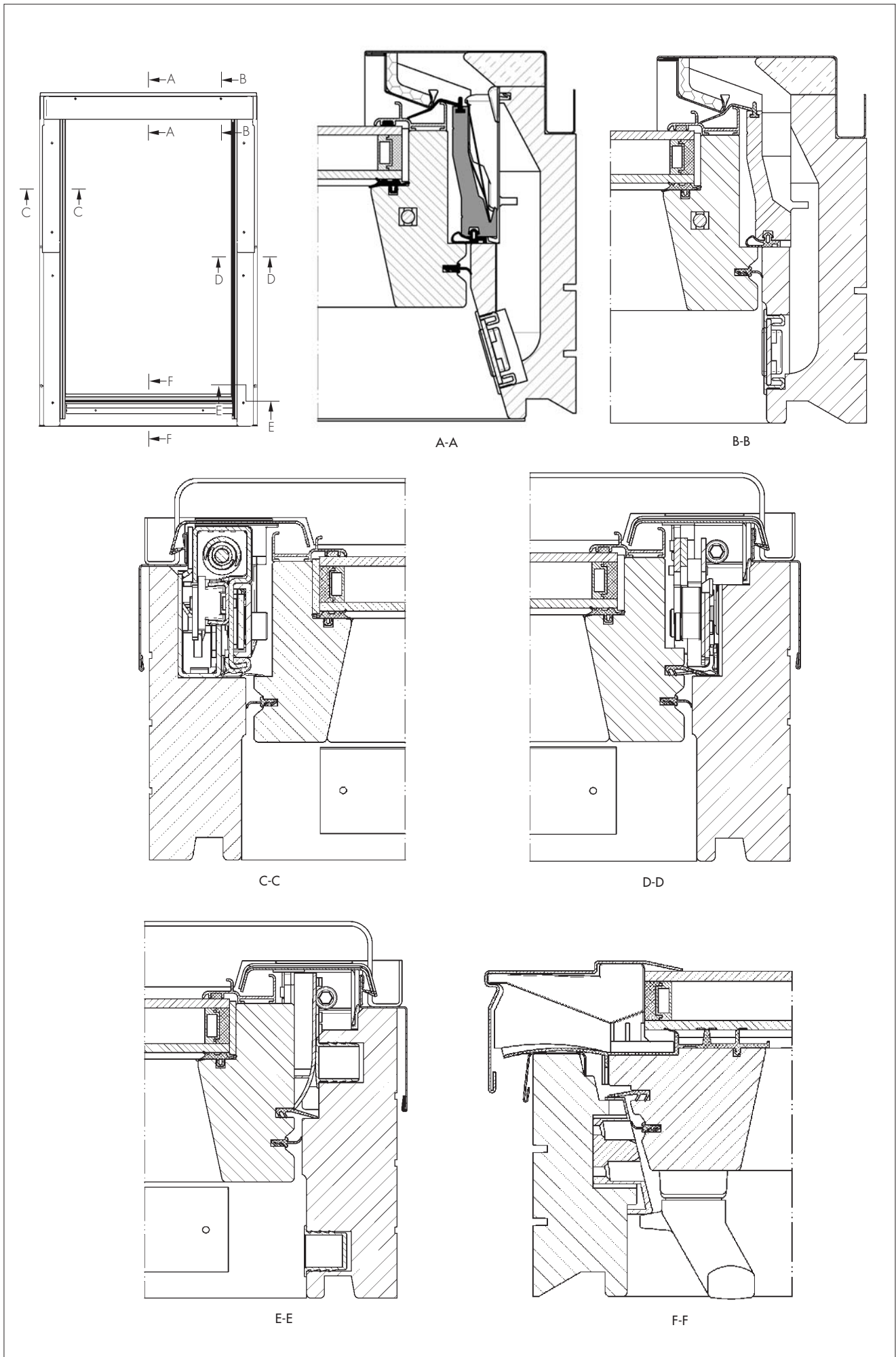
Figure 1 FPP preSelect Top-hung Roof Window cross-sections
